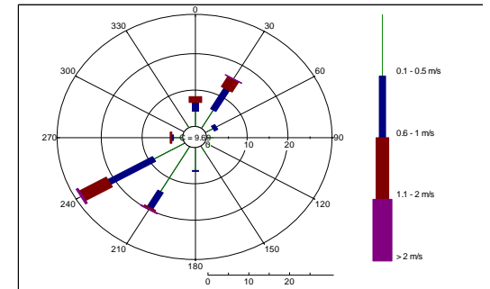
Wind Rose of BARC CAMS
