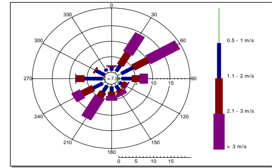
Wind Rose of BARC CAMS
