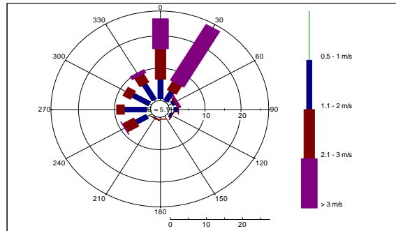
Wind Rose of Barisal CAMS
